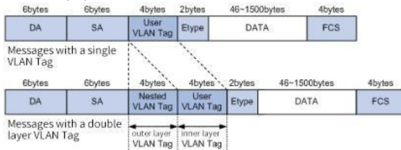
FIG. 3-127 QinQ's Packet Structure
