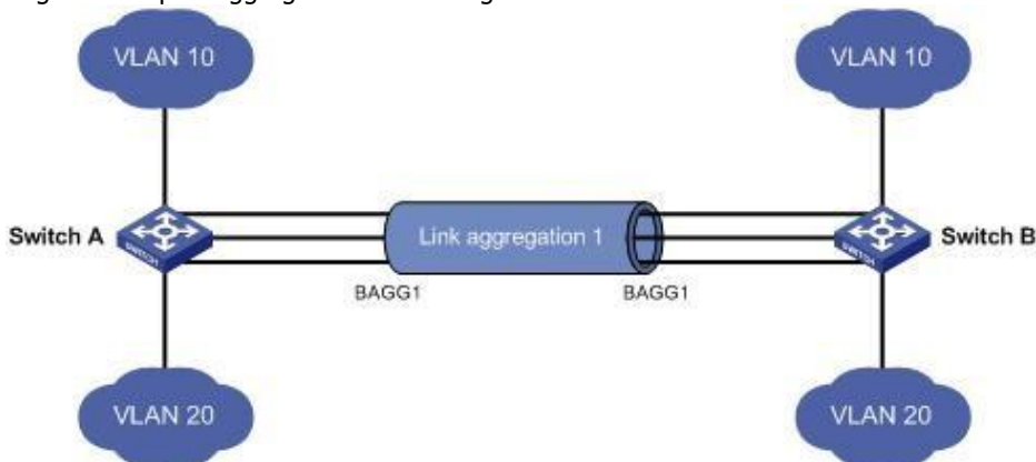
Figure 2-18 port aggregation networking model
