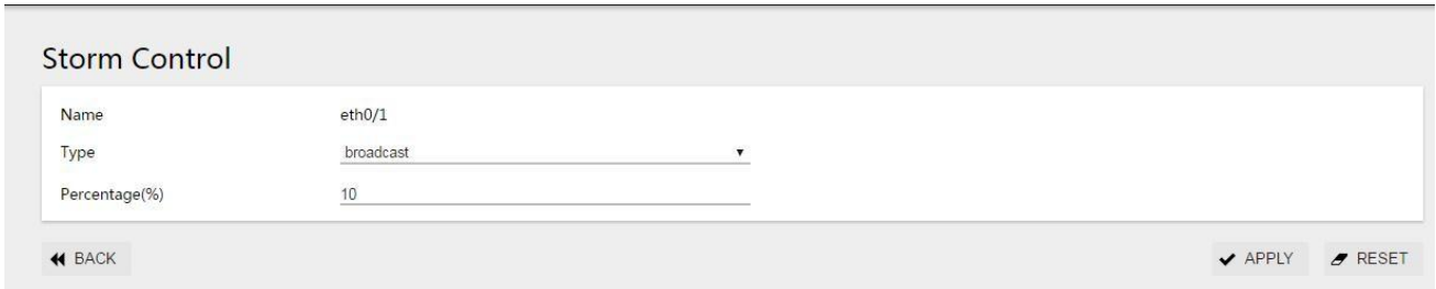
Figure 2-8 storm control configuration interface
