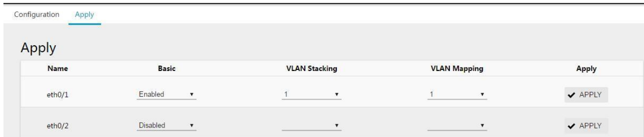
Figure 3-131 Configure the Type of QinQ Port
