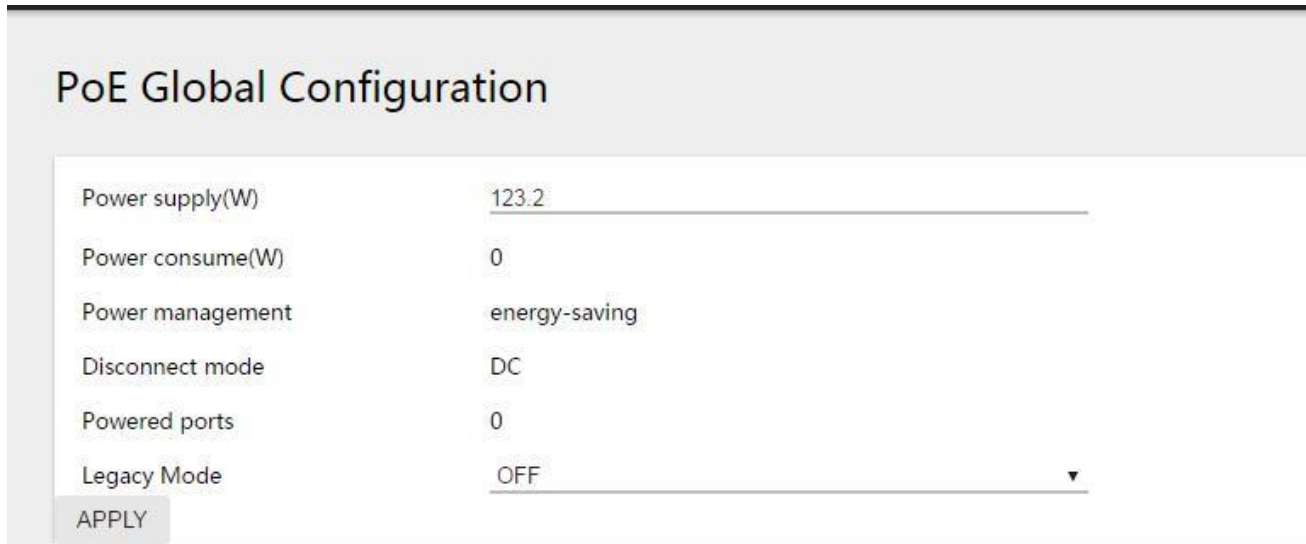
Figure 2-28 PoE global configuration
