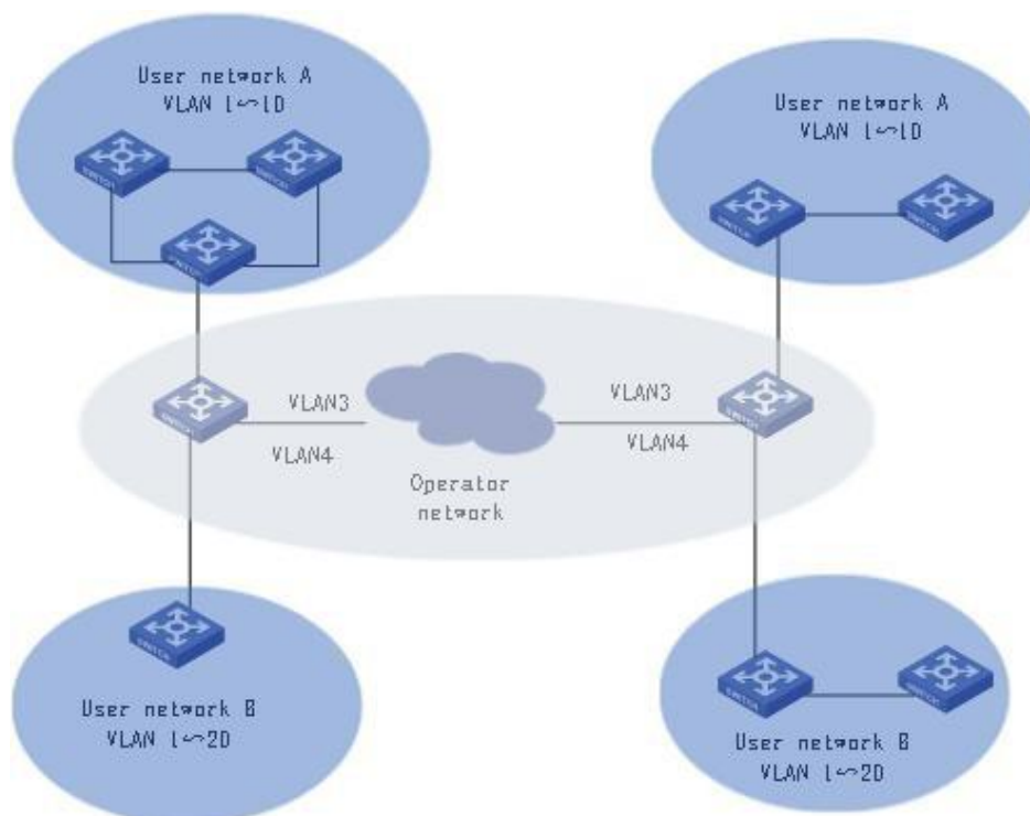
FIG. 3-126 QinQ Application Network Diagram
