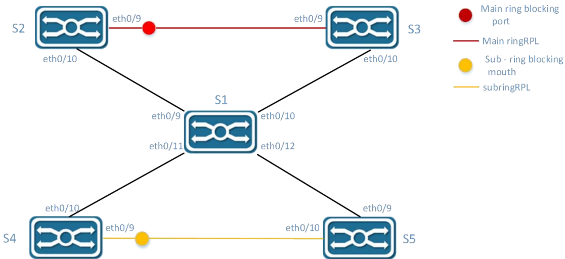
Figure 3-33 network topology
