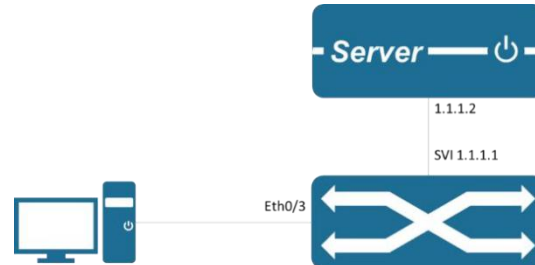
Figure 4-32 802.1X Authentication Typical Network Diagram
