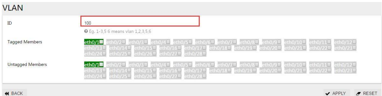
Figure 6-22 new VLAN interface
